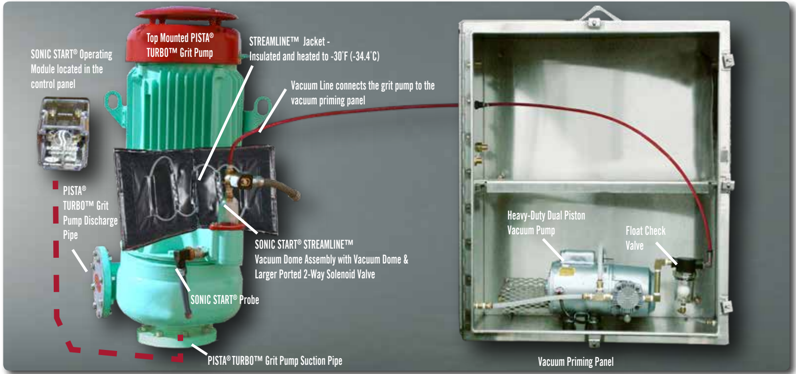
Shown above is the Top-Mounted PISTA® TURBO™ Grit Pump SONIC START® STREAMLINE™ Vacuum Priming System component diagram.
